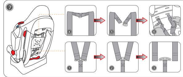
7. The shoulder belt height adjuster: before adjustment, remove baffle plate first. According to different heights of children, 4 levels of shoulder belt heights can be adjusted. Firstly, as shown in picture 1/2/3, separate the shoulder safety belt with strap yoke, and then according to 4/5, separate the shoulder belt with harness yoke and correspond to the appropriate harness slots to insert both of shoulder safety belts (see picture 6). Finally, connect both of the safety belts as shown in figures (3/2/1&5/4).
